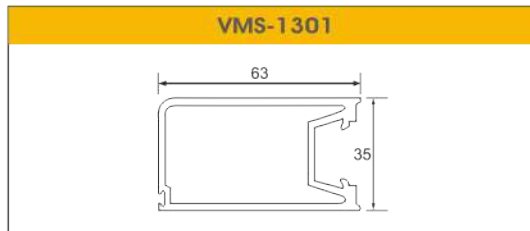
STILE DOOR FIX
