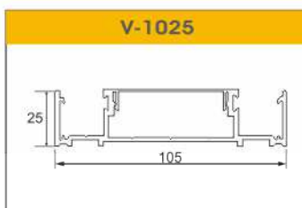
DOUBLE GLAZE SLIM FIX PROFILE FOR FIX PARTITION FINISH : MATT BLACK SIZE : 5000MM
