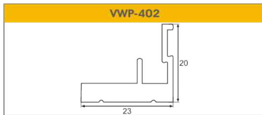
TOP AND BOTTOM HANDLE
