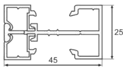
SINGLE GLAZE MALE FEMALE MIDDLE
