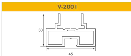
V-2001 TOP & BOTTOM PROFILE USED FOR SLIDING DOOR & OPENABLE DOOR
