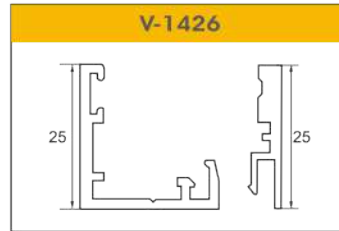
V-1426 SINGLE GLAZE 25*25 MALE FEMALE PRORILE FINISH : MATT BLACK CERAMIC SIZE : 3.00MTR, 3.66 MTR
