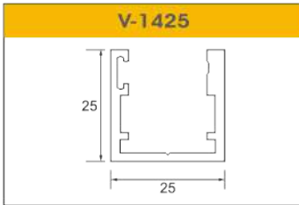
V-1425 SINGLE GLAZE 25*25 FIX PROFILE FINISH : MATT BLACK CERAMIC SIZE : 3.00MTR, 3.66 MTR
