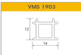
VMS 1903 T SECTION (10/12MM GLASS) COLOUR : MATT BLACK SIZE : 300 MM
