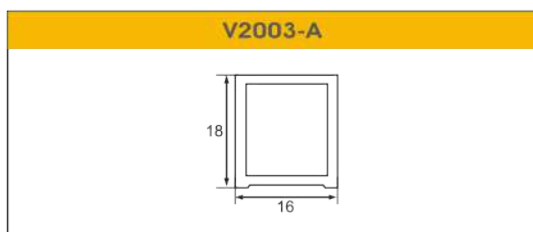
V2003-A 16X18 STICKING PROFILE USED FOR DOOR PATTERN
