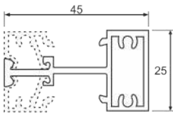
SINGLE GLAZE MALE FEMALE MIDDLE WITH SCREW FIXING GAP
