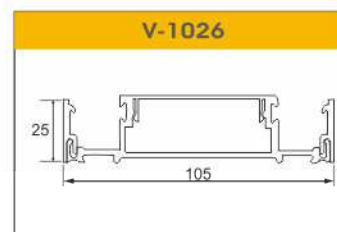
DOUBLE GLAZE SLIM MALE FEMALE PROFILE FOR FIX PARTITION FINISH : MATT BLACK SIZE : 5000MM
