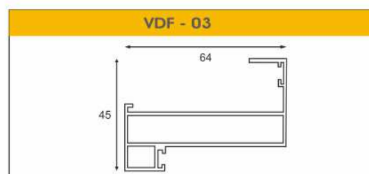
DOOR FRAME ( OUTSIDE OPENING )
