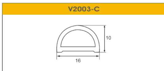
V2003-C ROUND STICKING PROFILE USED FOR DOOR PATTERN
