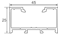
SINGLE GLAZE FIX PROFILE
