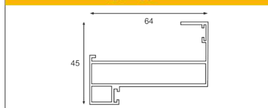
DOOR FRAME ( OUTSIDE OPENING )
