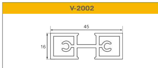
V-2002 DIVIDING PROFILE USED FOR HORIZONTAL AND VERTICAL ACTUAL PARTITION
