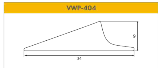
HANDLE FOR CURVE SHAPE PROFILE
