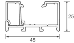
SINGLE GLAZE MALE FEMALE PROFILE
