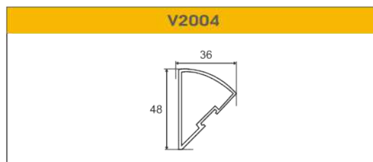
V2004 ROUND CORNER PIPE USED FOR CURVE CORNER IN FIX SLIDING
