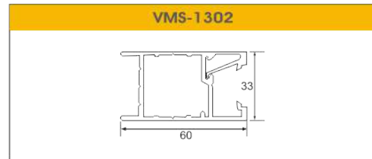
STILE DOOR MALE FEMALE
