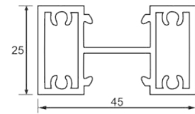
SINGLE GLAZE FIX MIDDLE WITH SCREW FIXING GAP
