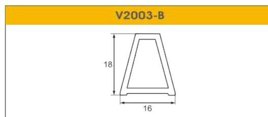
V2003-B 7 X 18 STICKING PROFILE USED FOR DOOR PATTERN
