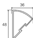
ROUND CORNER PIPE
