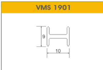
VMS 1901 I SECTION 3000 MM (10/12MM GLASS) COLOUR : MATT BLACK SIZE : 300 MM
